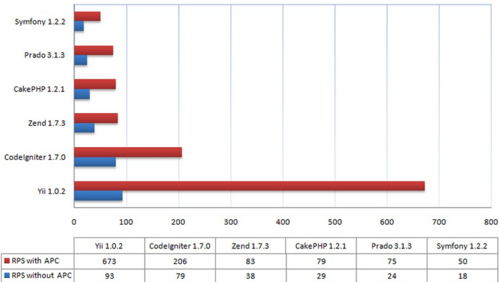
PHP Framework Performance Comparison
