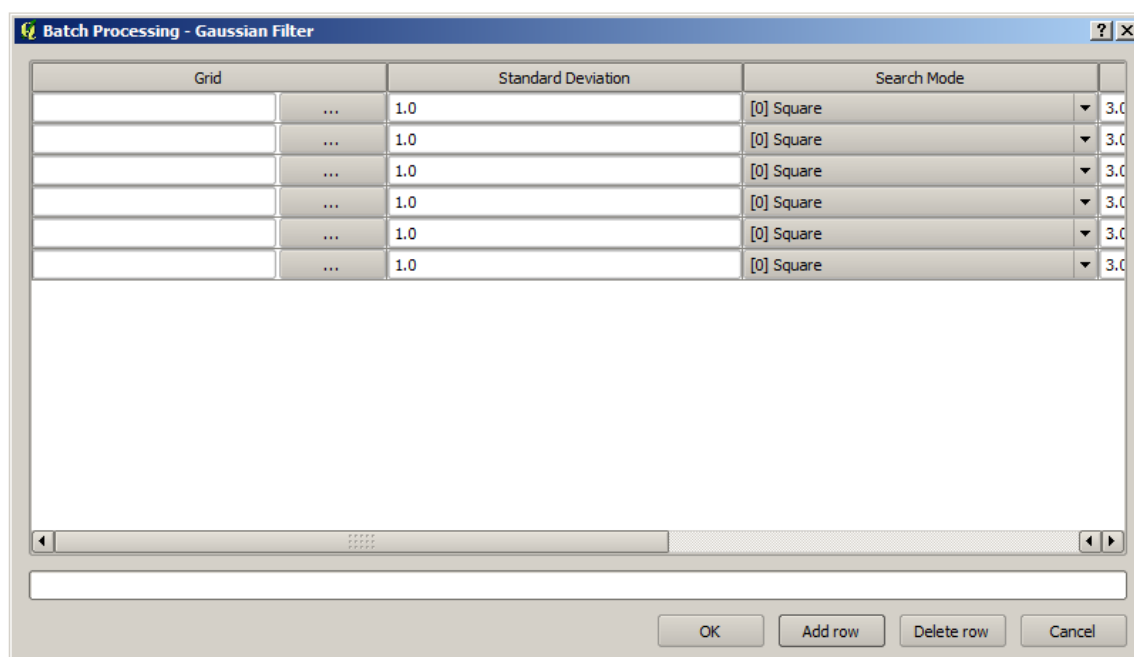
Figure 17.26: Batch Processing
